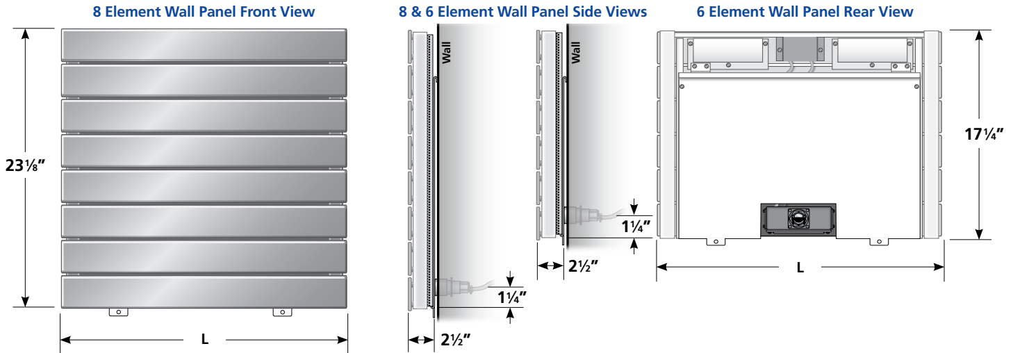
Runtal offers two wall panel sizes and three lengths.
